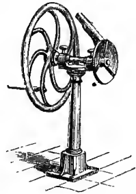
CHIPPING-MACHINE.
